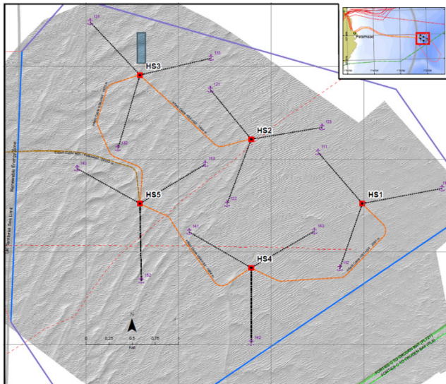
Hywind Field Layout
